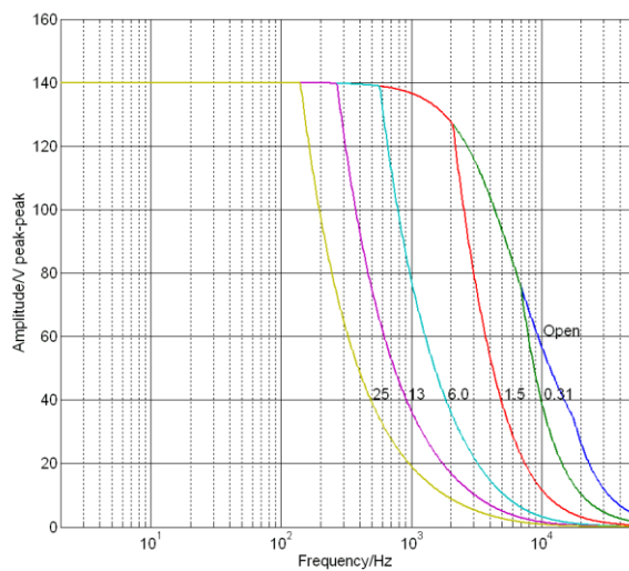
E-617: Operating limits (open loop) with various capacitive loads, capacitance values in μF
